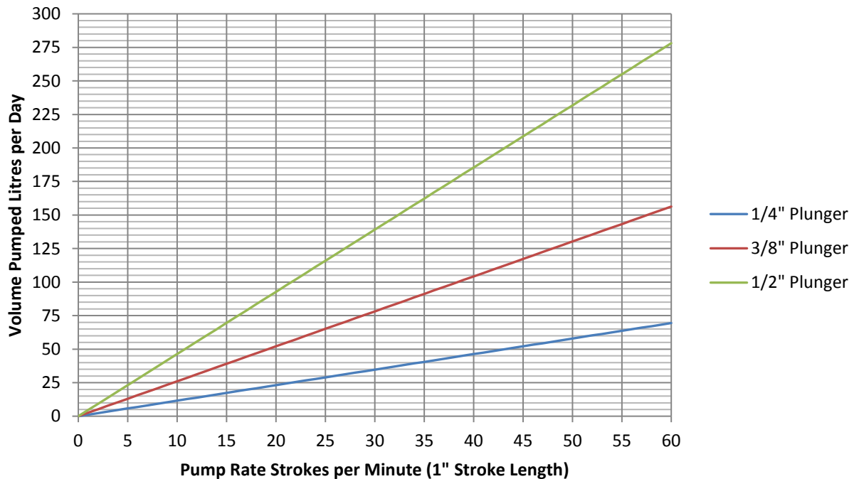
Electric Chemical Pump Volume Chart
